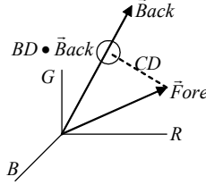
Figure 1. Distortion measurements in the RGB color space: \vec{Fore} denotes the RGB value of a pixel in the incoming frame that has been classified as foreground. \vec{Back} is that of its counterpart in the background.
